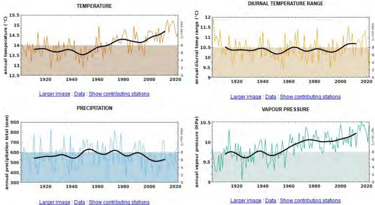
CRU TS 4.07 grid-box data for 37.75 S, 144.75 E
